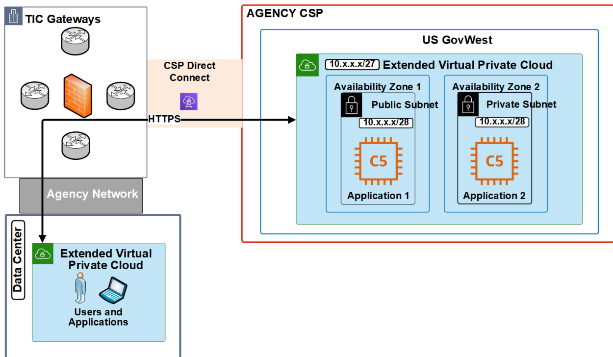
Figure 6. Generic use case of hybrid-cloud architecture.
